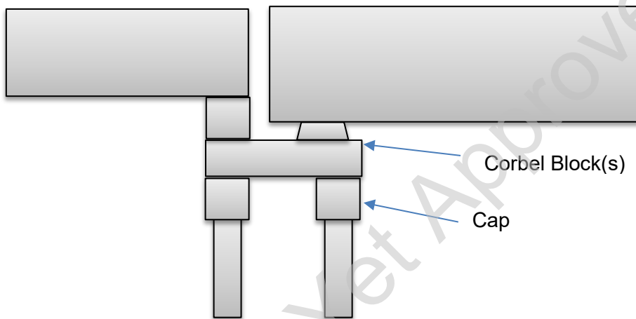
Figure 7-G-1. Example of Corbel Block
