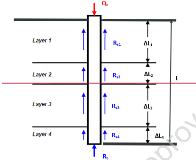
Figure 8-24-2. Idealized Geomaterial Layering for Computation of Geotechnical Resistances (after FHWA GEC 010, FHWA-NHI-10-016)
